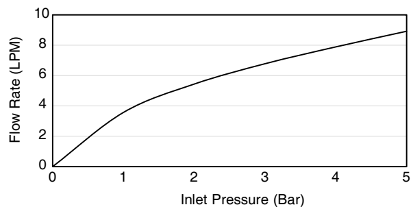
Flow Curve
