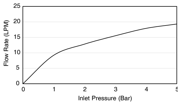
Flow Curve
