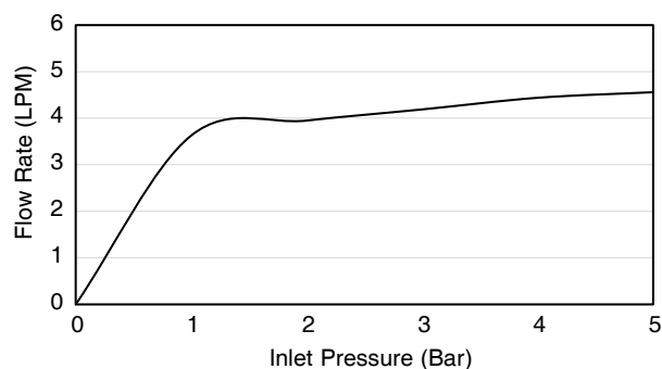
Flow Curve
