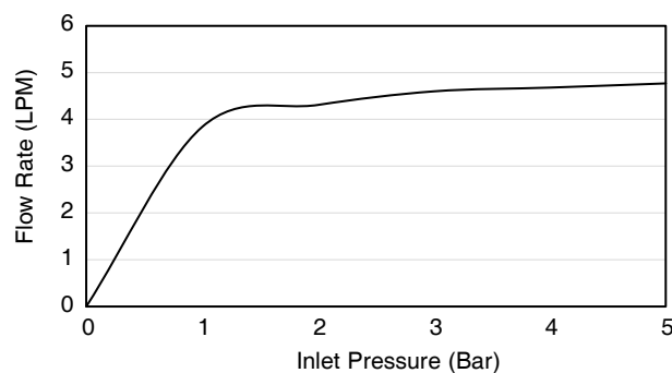
Flow Curve
