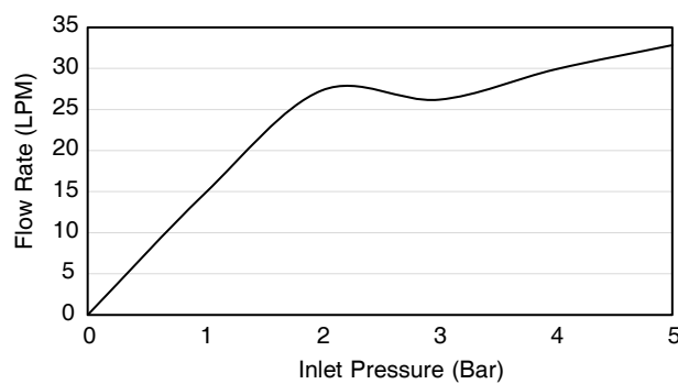
Flow Curve
